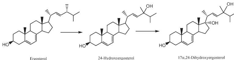
Figure 3. Proposed Sequence for the P450scc Catalyzed Transformation of Ergosterol with Structures of Expected Reaction Products
